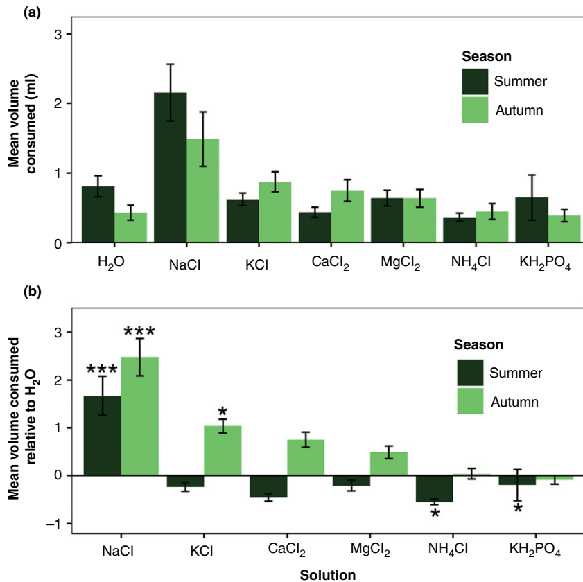
Fig. 3. (a) Mean volume change of each mineral consumed (ml) by all eight hives separated by season. Error bars are \pm 1 SE and show the variation in volume consumed for each trial within each season. There was no significant effect of season on the volume consumed; however, there was an effect of mineral solution. (b) Volume change for each mineral solution relative to the volume change of deionised water (negative control, x = 0.0 ), calculated for each field season. Anything above the baseline was preferred compared with deionised water, and anything below the baseline was avoided compared with deionised water. Bees significantly preferred sodium no matter the season. In the autumn, bees significantly preferred potassium. In the summer, bees significantly avoided nitrogen and phosphorus. Error bars are \pm 1 SE and show the variation in volume consumed for each trial within each season. (* P < 0.05 , *** P < 0.001 ). [Colour figure can be viewed at wileyonlinelibrary.com ].
