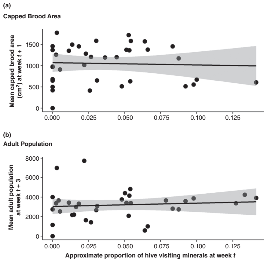
Fig. 4. (a) Approximate mean proportion of hives visiting minerals in week t and the mean capped brood area of hives in week t + 1 . (b) Approximate mean proportion of hives visiting minerals in week t and the mean adult population of hives in week t + 3 . Offsets were determined based on the honey bee life cycle (Winston, 1987). Although both analyses gave significant results, the near-zero pseudo- R^2 values indicate that the model explains our data only slightly better than a straight line.
