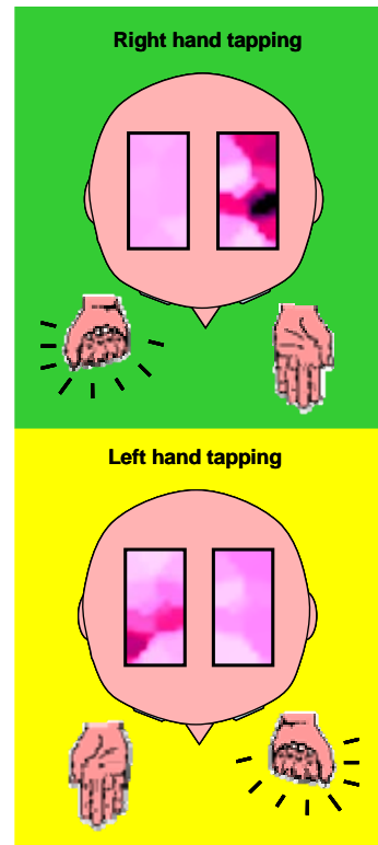
Fig. 4. Optical maps of right and left brain sides during right-hand tapping (top) and left-hand tapping (bottom). The brain side opposite to the tapping hand shows activation (the darker areas indicate a local increase in blood flow in response to brain activation).
