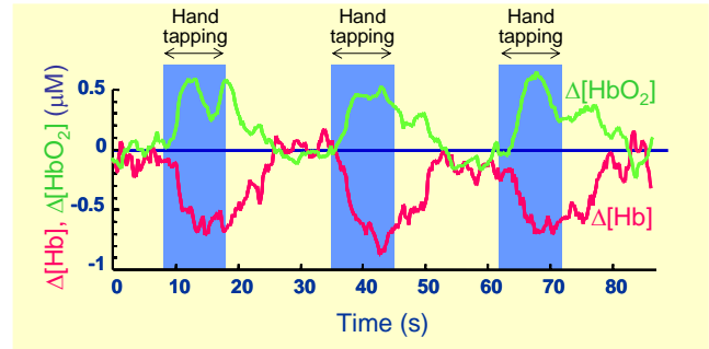
Fig. 3. The increase in the cerebral concentration of oxy-hemoglobin (positive \Delta[\text{HbO}_2] ) and the decrease in the cerebral concentration of deoxy-hemoglobin (negative \Delta[\text{Hb}] ) are the signatures of brain activation. These traces were recorded on the left motor cortex of a human subject during a right-hand-tapping protocol (hand tapping occurred during the periods indicated by the blue bars).
