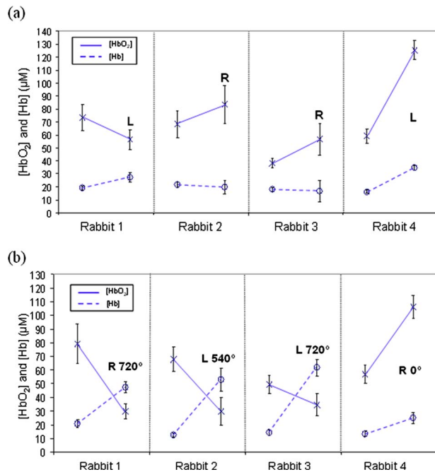
Fig. 3 Absolute values of concentrations of \text{HbO}_2 and \text{Hb} measured in testicular tissue for all four rabbits. Each line starts at the baseline value and ends at the postoperative value of [\text{HbO}_2] (continuous lines) and [\text{Hb}] (dashed lines) on (a) the control testes or (b) the experimental testes. Here L refers to left and R refers to right testicle with associated degrees of torsions.
