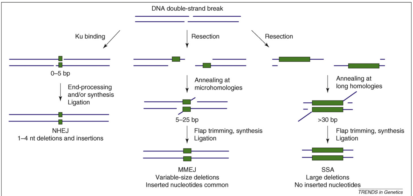
Figure 1. Comparison of NHEJ, MMEJ and SSA pathways in S. cerevisiae . During NHEJ repair of a DSB, the Ku70–Ku80 heterodimer binds, preventing DNA end resection. Repair proceeds by annealing at short microhomologies (green boxes), fill-in by Pol \alpha and ligation using DNA ligase IV, resulting in small deletion and insertion products. Both MMEJ and SSA require end resection or unwinding to reveal homologous sequences, although the length of homology required for MMEJ (5–25 bp) is shorter than for SSA. SSA and MMEJ also require 3' flap cleavage before fill-in synthesis and ligation. Whereas MMEJ products can contain inserted nucleotides, these are never observed in SSA. Notably, although the three pathways share some common genetic requirements, overall they are distinct (Table 1).
