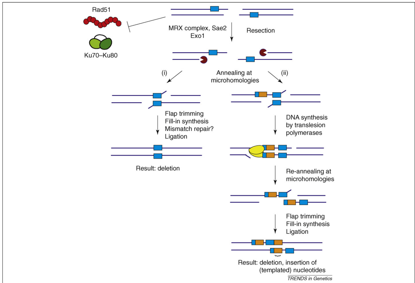
Figure 2. Model for MMEJ and alternative end-joining repair. During the initial stages of MMEJ, Ku70–Ku80 (green) and Rad51 (red), which inhibit MMEJ, are prevented from binding or are removed. This enables 5′–3′ resection by the MRX complex, Sae2 and Exo1 (indicated by dark red partial circle) that reveals microhomologous sequences (blue boxes). These microhomologies transiently and dynamically anneal to each other. (i) In cases in which the annealing is stable, repair is completed by flap trimming, fill-in DNA synthesis and ligation, resulting in a deletion relative to the original sequence. Mismatch repair is not required for MMEJ, although it might have a supporting role. (ii) Alternatively, one or more translesion polymerases (yellow) can extend the annealed sequences (represented here by orange–blue boxes) using templated error-prone synthesis. Dissociation of the initial microhomologies and realignment at other microhomologous sequences, followed by flap trimming, fill-in DNA synthesis and ligation completes repair, resulting in a deletion plus insertion event. Many variations and iterations of (ii) can hypothetically occur, resulting in complex insertion–deletion junctions.
